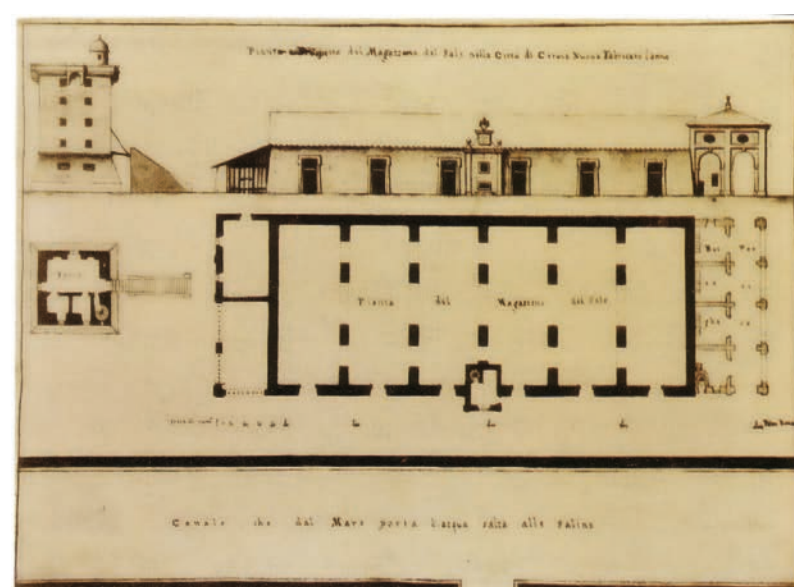
Cervia (RA), "Magazzino Torre" (Tower warehouse): plan and section of the warehouse (from History of Cervia , vol. II, Rimini 1998, Album Imperiali, private collection)
